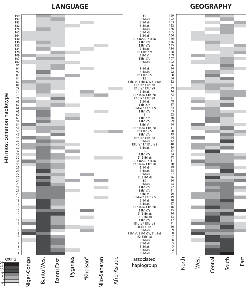
Fig. 4 Patterns of haplotype sharing. Heat plots showing the count of the most common haplotypes from 11 STRs (DYS19, DYS389I, DYS389II, DYS390, DYS391, DYS392, DYS393, DYS437, DYS438, DYS439, and the sum of DYS385a/b) shared among at least three individual groups. Individual groups are combined into metagroups according to their linguistic affiliation (left) and geographic location (right); the same heat plot, but for single groups, is reported in supplementary figure 5 (Supplementary Material online) .
