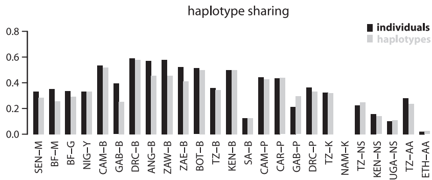
Fig. 5 Proportion of shared haplotypes. Histogram of the proportion of shared haplotypes between one group and all other groups based on 11 STRs. Black bars represent the proportion of all individuals sharing their haplotype (with any of the other groups) over the total number of individuals in a group; gray bars represent the proportion of unique shared haplotypes over the total number of haplotypes detected in a group.
