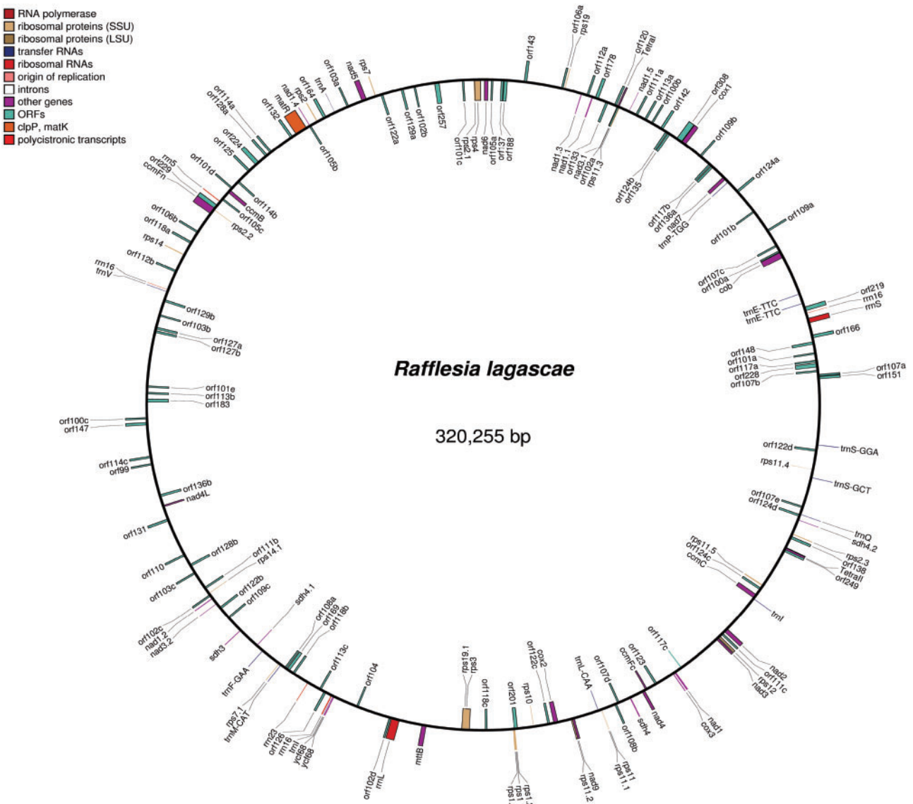
Fig. 2. Draft structure of R. lagascae mitochondrial genome. The gene positions indicated are based on the assumption of synteny with Ricinus (GenBank accession number HQ874649; Rivarola et al. 2011). The coordinates and encoded products of the specific genes are shown in supplementary table S1, Supplementary Material online. Although depicted as a complete circular genome, it should be stressed that this is a draft assembly with 213 gaps and that portions of the mitochondrial sequence remain unassembled.
