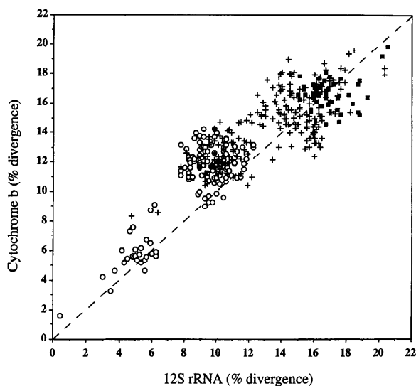
FIG. 2.—Observed sequence divergence of 12S rRNA (transitions and transversions in stems, transversions in loops) versus cytochrome b (conservative substitutions) for 406 pairwise comparisons encompassing 29 taxa. Empty circles represent comparisons between Cetacea and Artiodactyla, black stars represent comparisons between Cetacea + Artiodactyla and other eutherian taxa, and black squares represent comparisons between the two Marsupialia and eutherian taxa. The dotted line represents the bisecting line.
